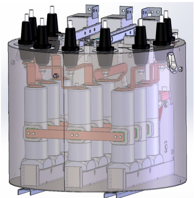
Trayer 100 series Solid Dielectric Load Break Switch 25kV, 600A, 3 ways, 3 ways switched Submersible Vacuum Load Break Switch shown with optional visible disconnect and motor operators
