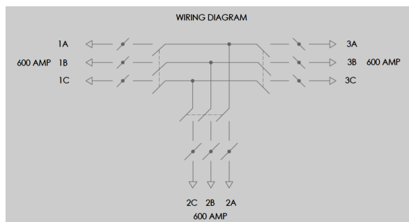
One Line Diagram
